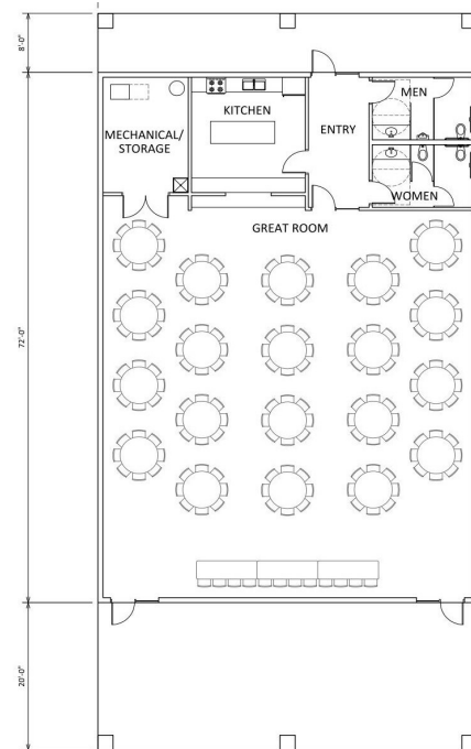
FLOOR PLAN - OPTION 2
